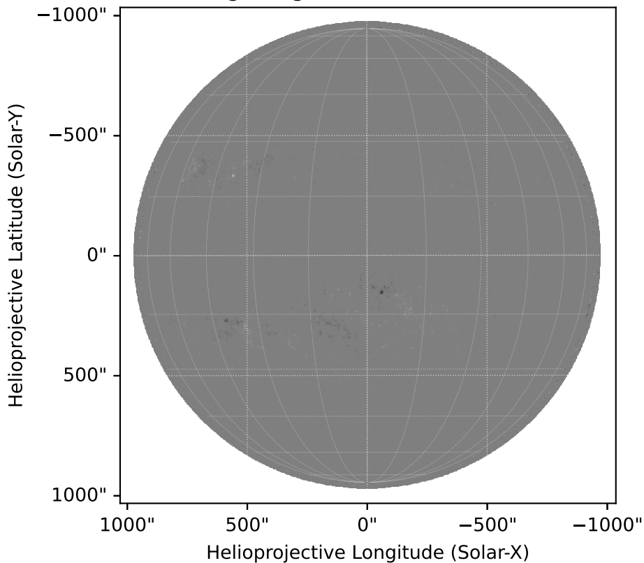
HMI magnetogram 2011-06-07 06:32:11
