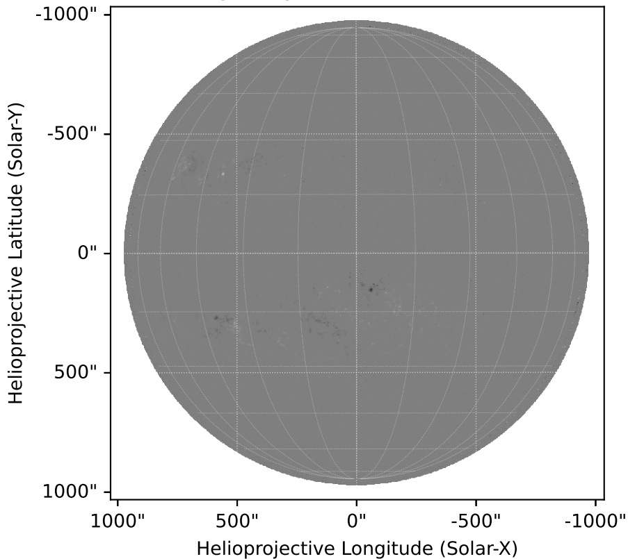
HMI magnetogram 2011-06-07 06:32:11
